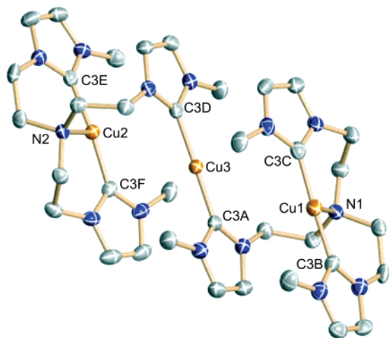
Figure 1. Solid-state molecular structure of complex [(\text{TIMEN}^{\text{Me}})_2\text{Cu}_3](\text{PF}_6)_3 \cdot 2.5\text{CH}_3\text{CN} ( 10 ). Hydrogen atoms, anions, and solvent molecules are omitted for clarity; thermal ellipsoids are at 50% probability. Selected bond lengths (Å) and angles (deg): Cu(1)–C(3B) 1.901(4), Cu(1)–C(3C) 1.894(5), Cu(1)–N(1) 2.365(3), Cu(2)–C(3E) 1.892(4), Cu(2)–C(3F) 1.891(4), Cu(2)–N(2) 2.371(3), Cu(3)–C(3A) 1.909(4), Cu(3)–C(3D) 1.910(4), C(3B)–Cu(1)–C(3C) 172.54(19), C(3E)–Cu(2)–C(3F) 166.50(17), C(3A)–Cu(3)–C(3D) 178.74(17).
